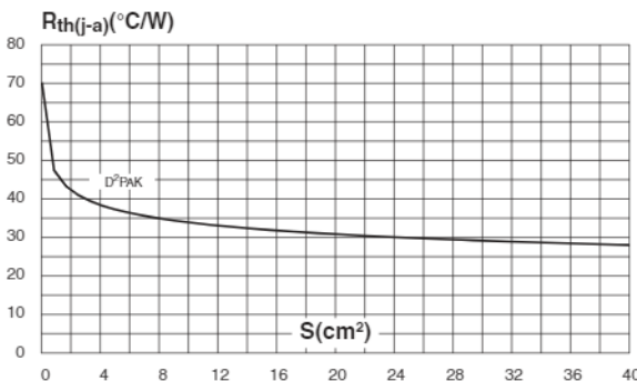
Figure 11: D 2 PAK Thermal resistance junction to ambient versus copper surface under tab (printed circuit board FR4, copper thickness: 35 \mu\text{m} )
